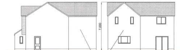
west elevation
